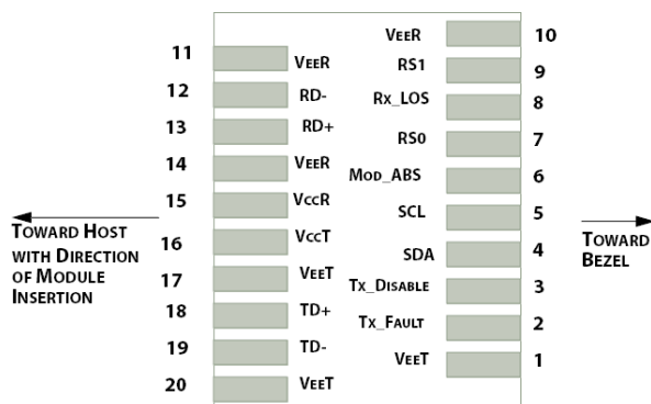
Figure1.Electrical Pin-out Details
