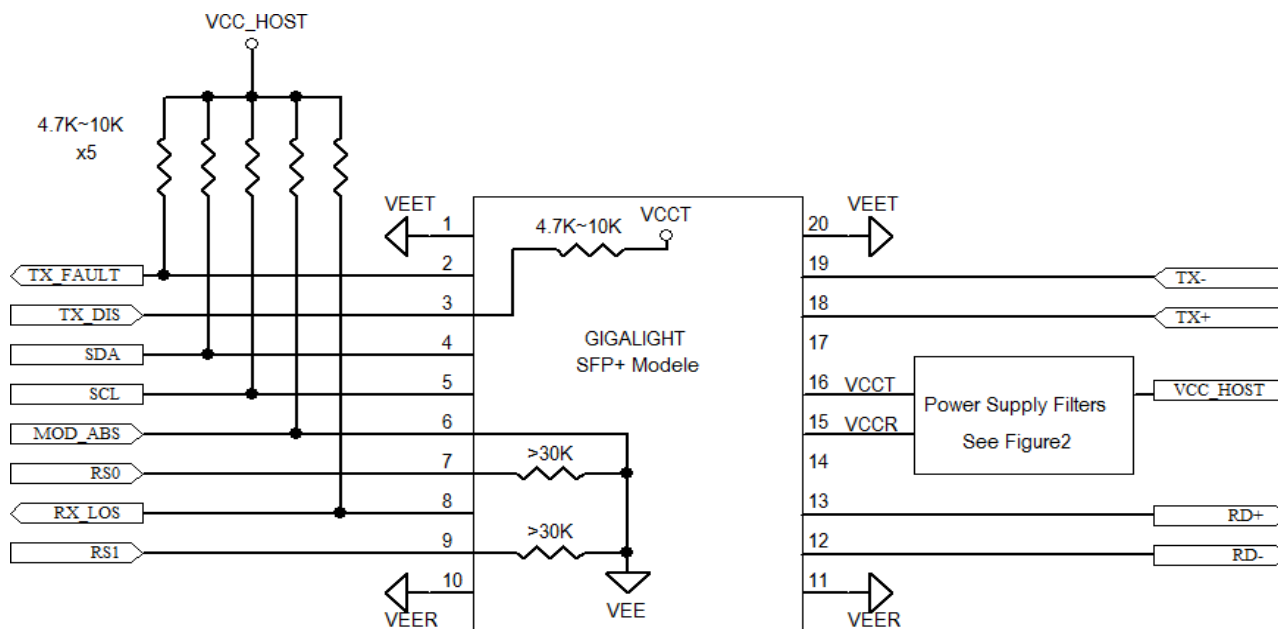
Figure3. Host-Module Interface
